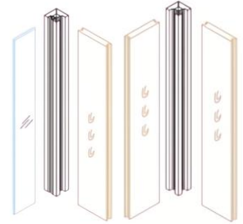
CORNER CONNECTION
