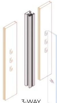
3-WAY CONNECTION
